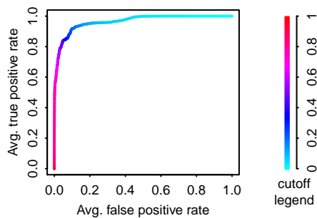
Figure 1. ROC plot for all 102 validation runs, averaged along cutoffs.
