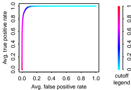
Figure 1. ROC plot for all 248 validation runs, averaged along cutoffs.
