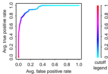
Figure 1. ROC plot for all 71 validation runs, averaged along cutoffs.
